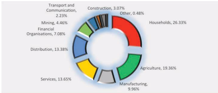
Figure 24: Sectoral Distribution of Credit as at December 2018
