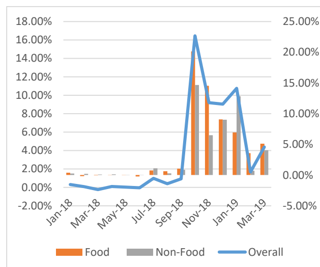
Figure 14: Annual Inflation (%)
